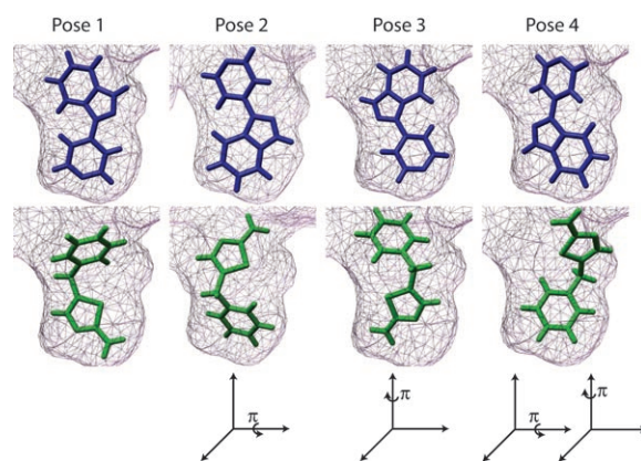
Figure 3. Binding orientations for ligands L_A and L_B . From the binding pose of the high-resolution crystal structure (pose 1), other possible binding orientations were generated by rotating the ligands by 180° around the y or the z axis, or both (poses 2–4). The possible binding orientations for L_A (blue model) and L_B (green model) are shown with the protein pocket indicated as an exclusion surface.
