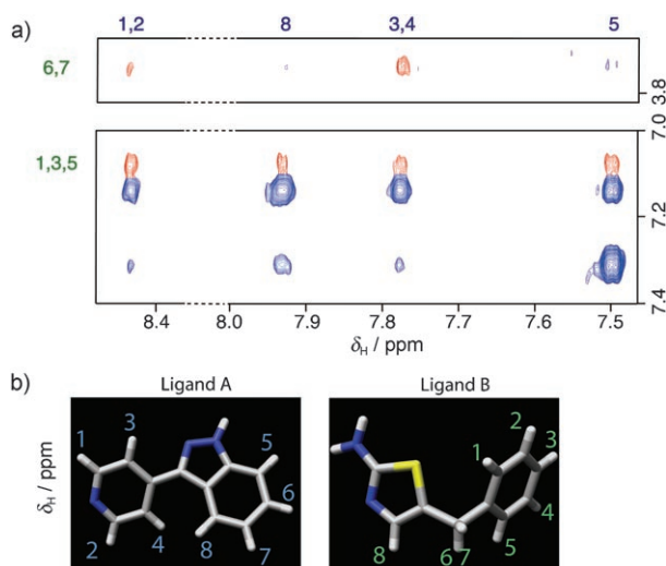
Figure 2. Experimental INPHARMA peaks: a) Region of the NOESY spectrum recorded for a mixture of 30 \mu\text{M} PKA, 150 \mu\text{M} L_A , and 450 \mu\text{M} L_B at 800 MHz for a mixing time of \tau_m = 600 ms. Intramolecular transfer NOEs: blue; intermolecular "INPHARMA" peaks: red. b) Chemical structures of L_A and L_B , the PKA inhibitors used in this study.
